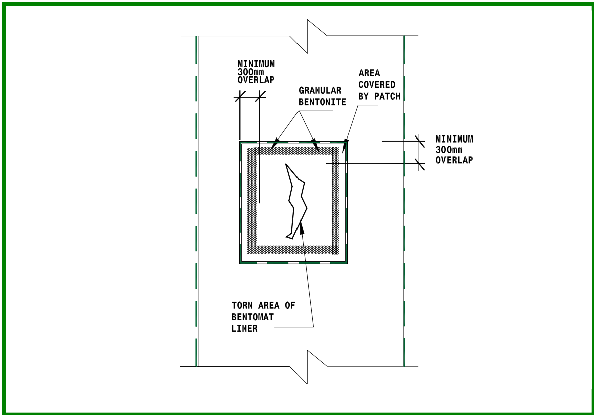
Figure 7. Damage repair by patching.
