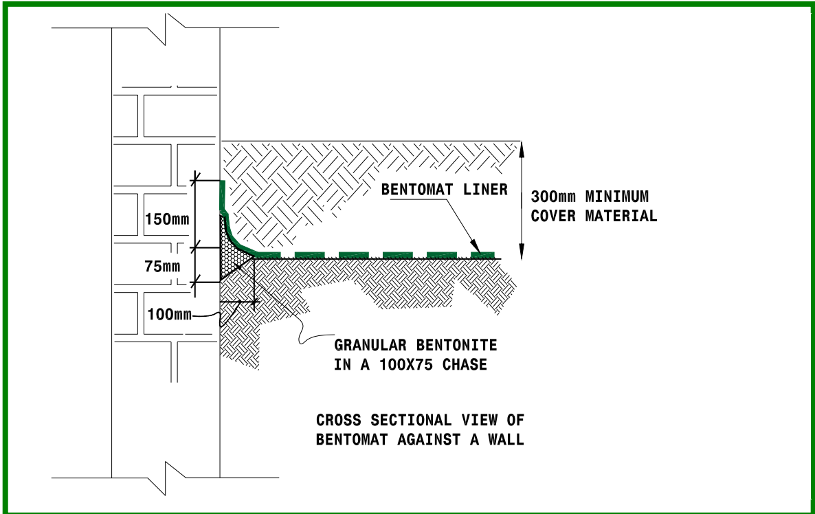
Figure 6. Cross-section of GCL against an embedded structure or wall.
