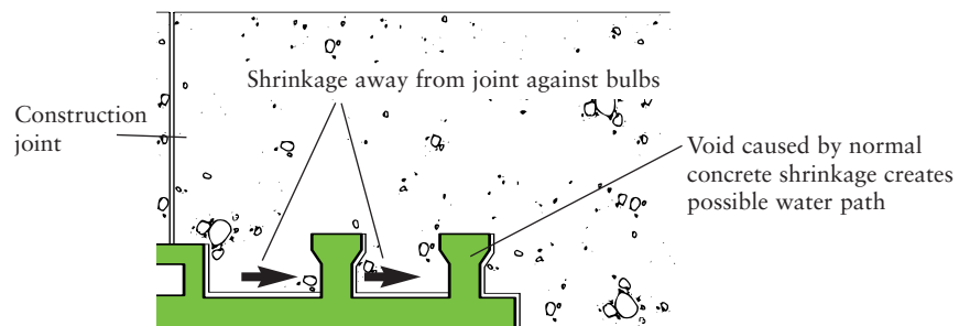
Conventional Waterstop
